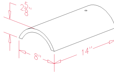
USED FOR STARTING COVER TILE
