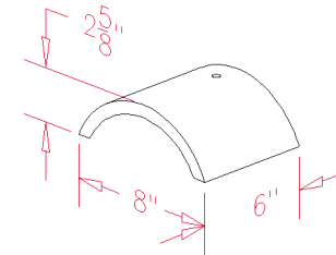
USED FOR DOUBLE EAVES
