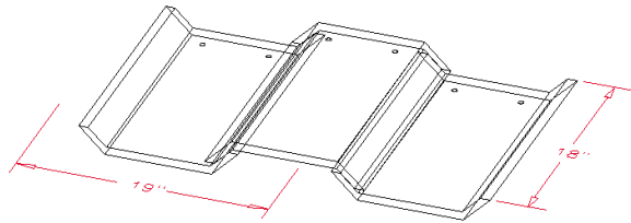
ITALIAN PANS WITH ITALIAN COVERS 102 Pieces/Sq. (3" Headlap) Approx. 1040 Lbs./Sq.
