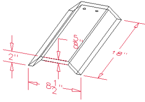
BERKELEY COVER (TURN OVER FOR PAN)
