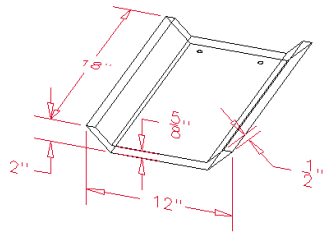
ITALIAN PAN (TURN OVER FOR COVER)
